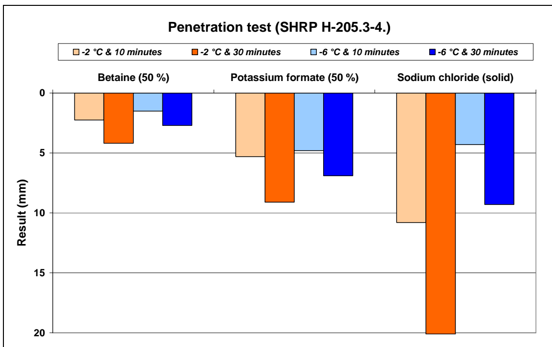
Figure 1 – Results of the penetration test made on betaine, potassium formate and sodium chloride.[1] [2]
