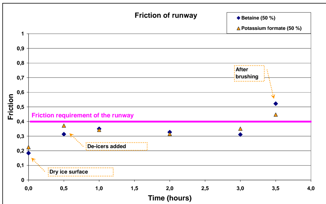
Figure 3 – Friction test results. The effect of brushing on friction is clearly visible in the results. However, no differences between these agents were recognized; both chemicals passed the requirement. [3]
