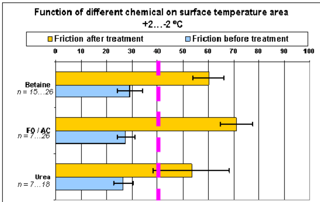
Figure 5 – Friction levels with 95 % confidence intervals of different chemicals when anti-skid treatment is being performed. Friction requirement of the runway is 40 in Finland. [4]
